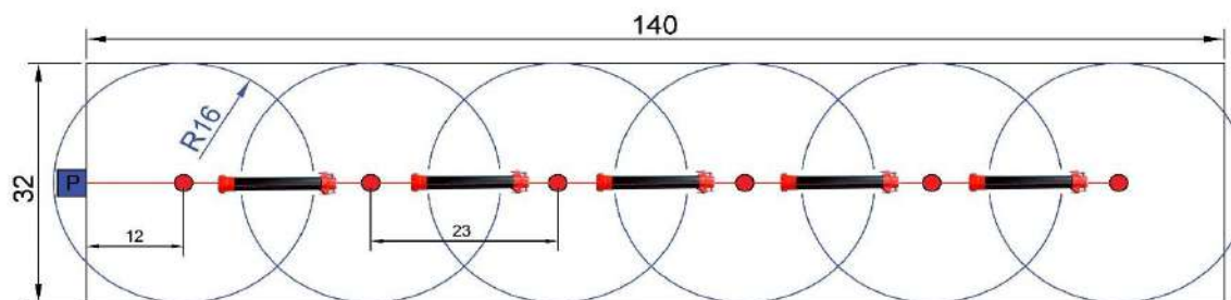
Atom22 (8mm Nozzle ) X 6 Sprinkler - 10 HP High Pressure Motopump Total Irrigated Area : 4500m 2 - Irrigation Pipe Diameter : 75mm
