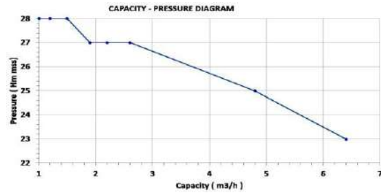
6,5 HP Gasoline Motopump Self Suction
