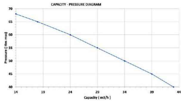
20 HP Gasoline Motopump High Pressure - Electric Start
