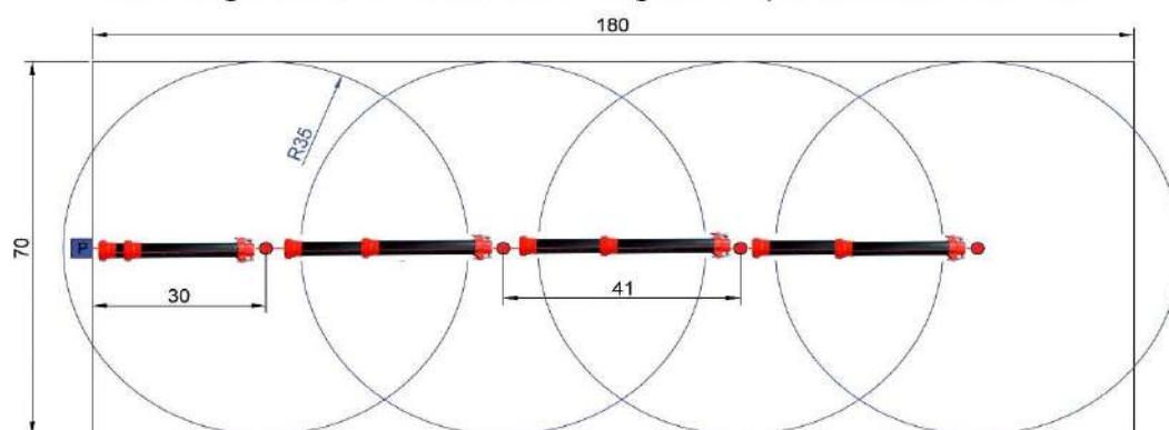
JET50 (20mm Nozzle) X 4 Sprinkler - DCR125 Tractor PTO Pump Total Irrigated Area : 12.500m 2 - Irrigation Pipe Diameter : 110mm
