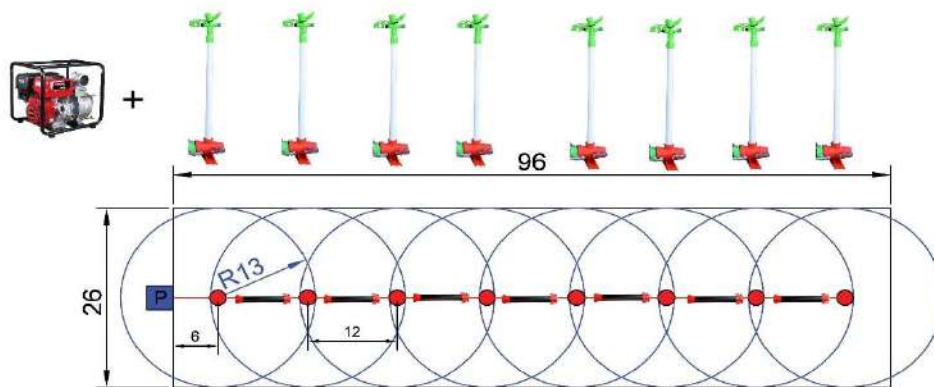
Atom15 LF ( 4.5X2.5 ) X 8 Sprinkler - 6.5 HP High Pressure Motopump Total Irrigated Area : 2500m 2 - Irrigation Pipe Diameter : 63mm
