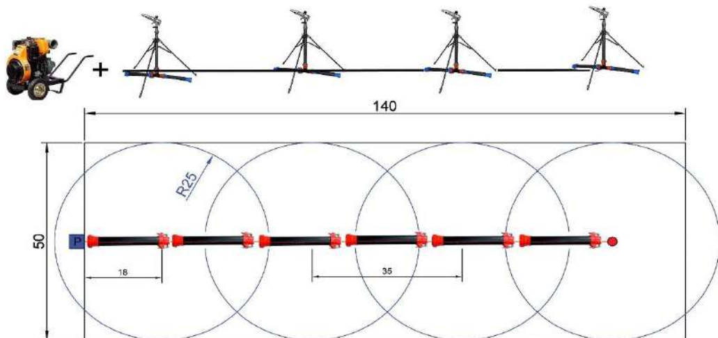
ATOM35 (14mm Nozzle) X 4 Sprinkler - 17 HP Diesel Motopump Total Irrigated Area : 7000m 2 - Irrigation Pipe Diameter : 90mm
