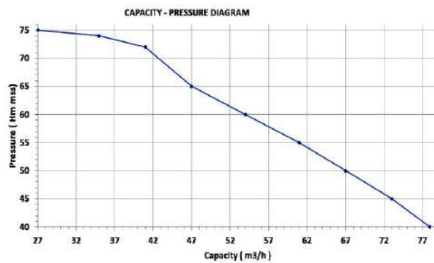
20 HP Gasoline Motopump High Pressure - Electric Start
