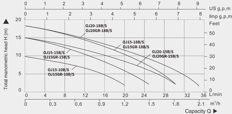
PERFORMANCE CHART
