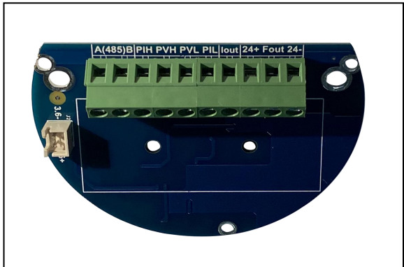
Four-wire 485 communication wiring universal(old models)
