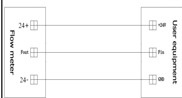
Three-wire pulse output wiring with display (24V power supply)
