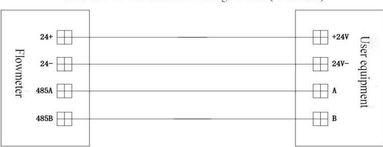
Four-wire 485 communication wiring universal(old models)
