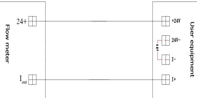
Two-wire 4-20mA current output connected to totalizer (two-wire to four-wire)
