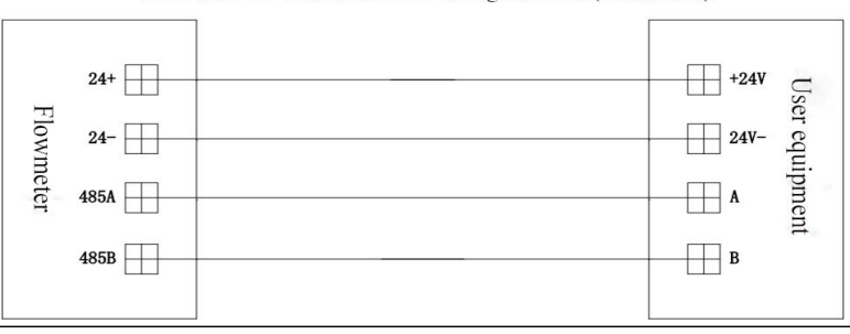
Four-wire 485 communication wiring universal(old models)
