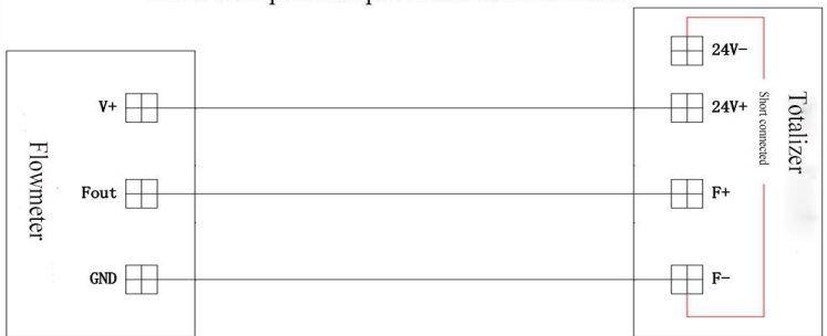
Three-wire pulse output connected calculator
