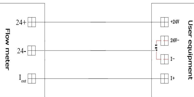
Three-wire 4-20mA current output totalizer
