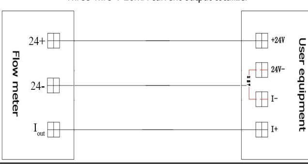
Three-wire 4-20mA current output totalizer
