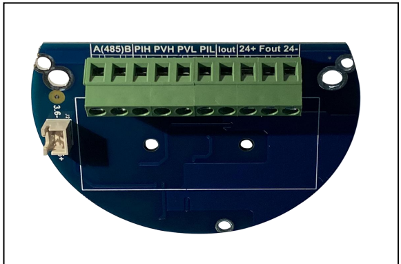
Four-wire 485 communication wiring universal(old models)
