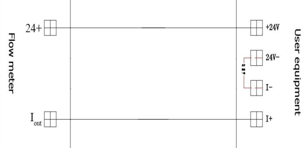
Three-wire 4-20mA current output totalizer
