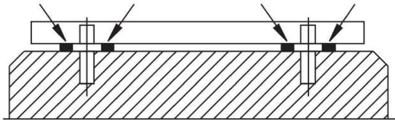
Figure 4 fitting the shims
