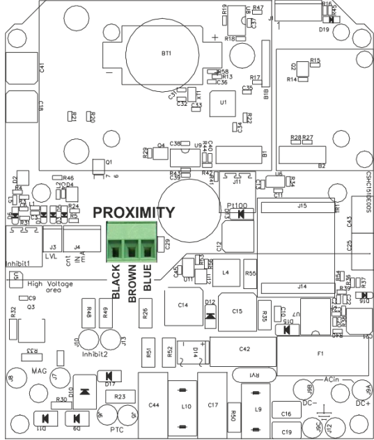
Proximity sensor's connection
